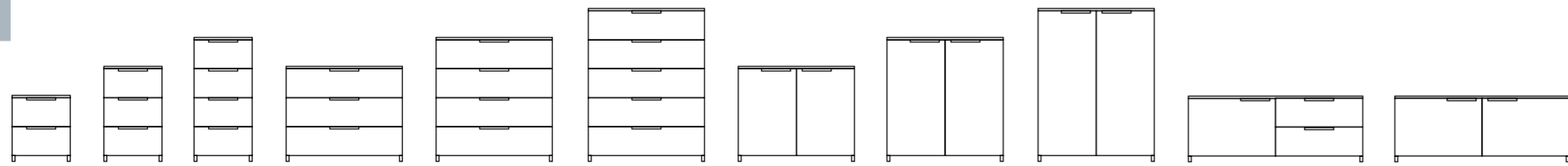
block 01 400x400x460 block 02 400x400x660 block 03 400x400x860 block 04 800x400x660 block 05 800x400x860 block 06 800x400x1060 block 07 800x400x660 block 08 800x400x860 block 09 800x400x1060 block 10 1200x500x460 block 11 1200x500x460
